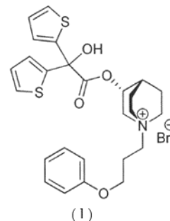
Aklidinium Bromid
