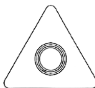
15.2
