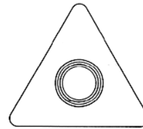
22.2
