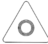
20.2
